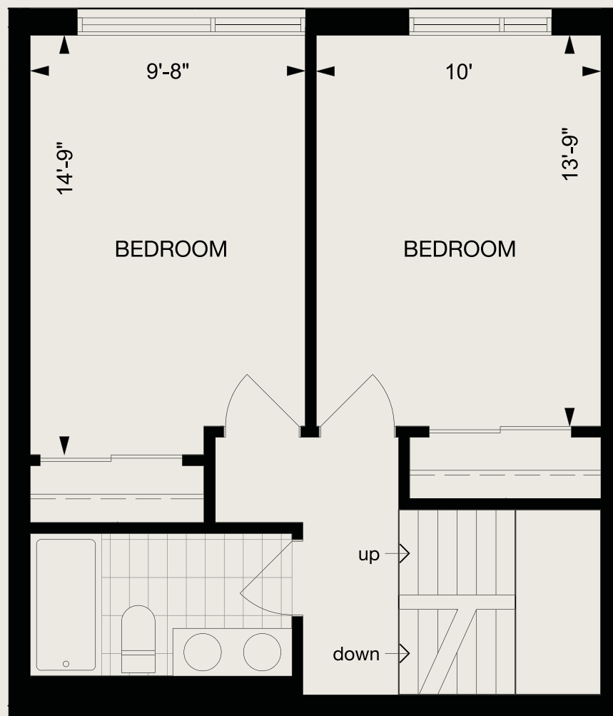
SECOND FLOOR
